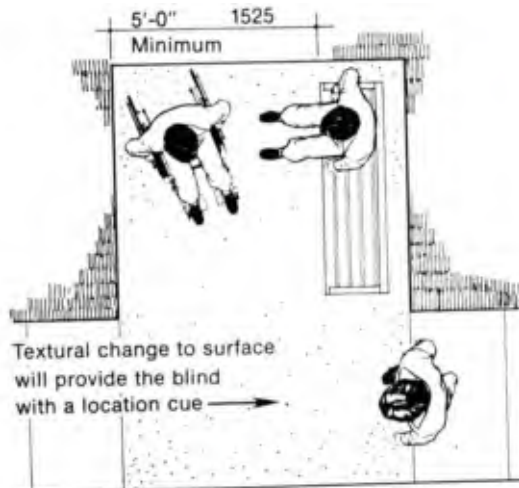
Figure 3.7.4 Space requirements for wheelchairs adjacent seating
