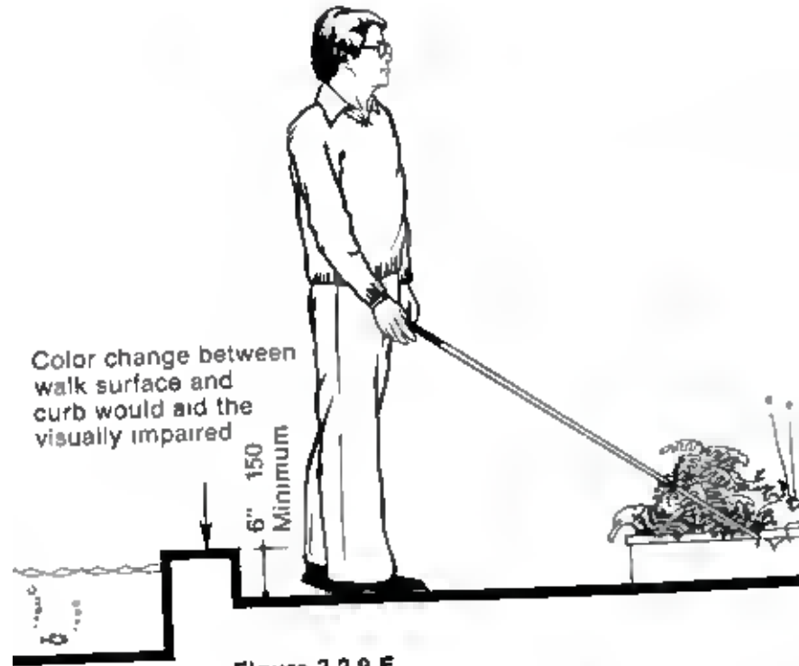
Figure 3.2.9 E Locatable barriers around pools and landscaping
